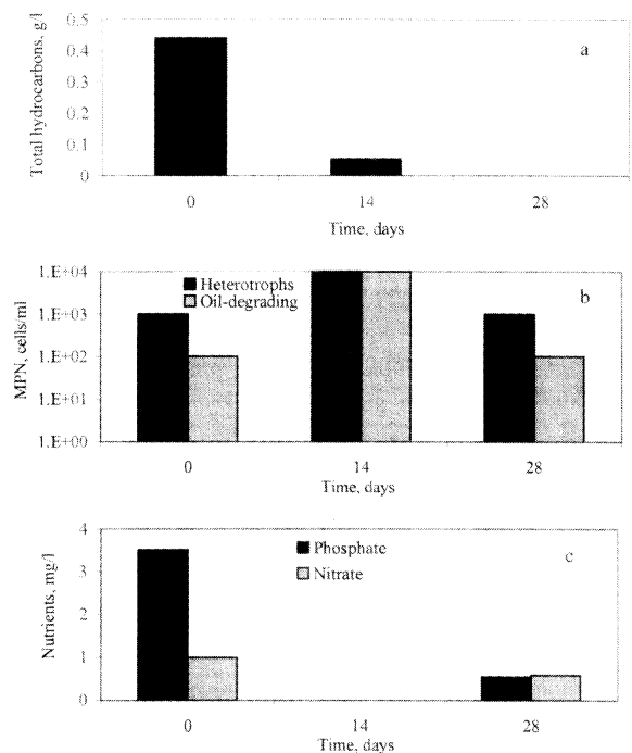
Figure 1. Dynamics of concentrations of total hydrocarbons (a), hydrocarbon-degrading and heterotrophic bacteria (b), phosphate and nitrate (c) during the 'Rhoder' bioremediation of bay of the River Chernaya.
